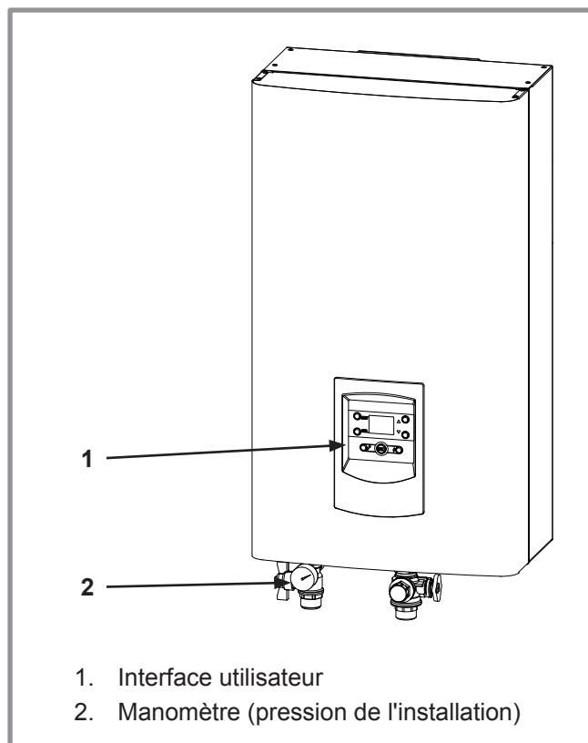
figure 3 - Compact Combi
